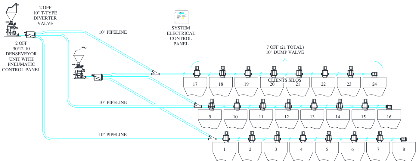
System Flow Layout
