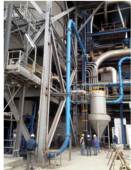
Power station boiler building – system 3
